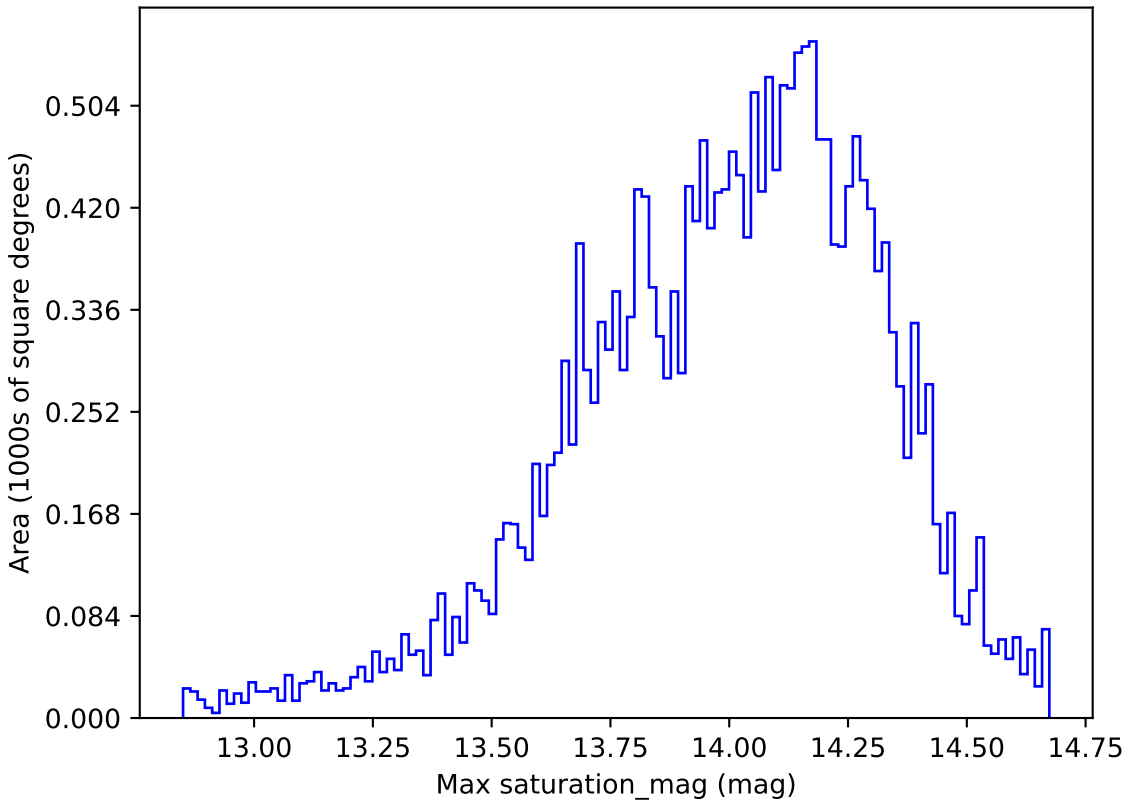
too_100_4v3.4_10yrs All sky u band: Max saturation_mag
