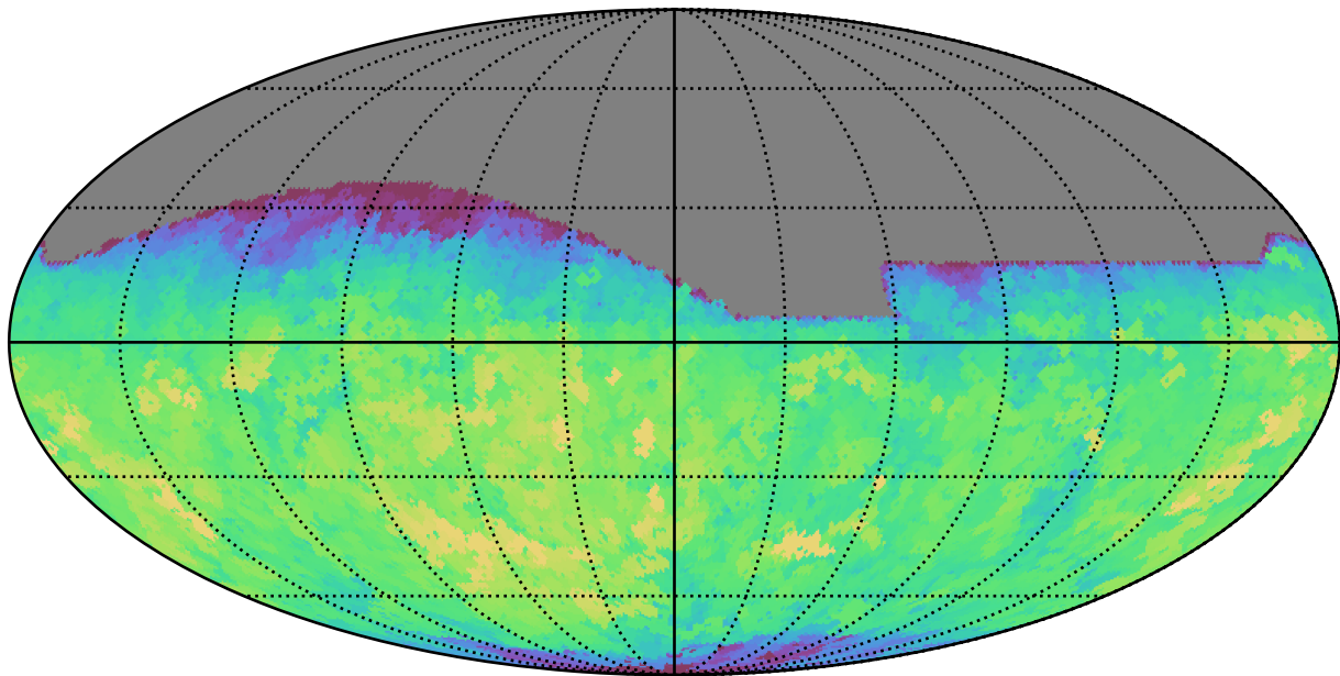
too_100_4v3.4_10yrs All sky r band: Max saturation_mag
