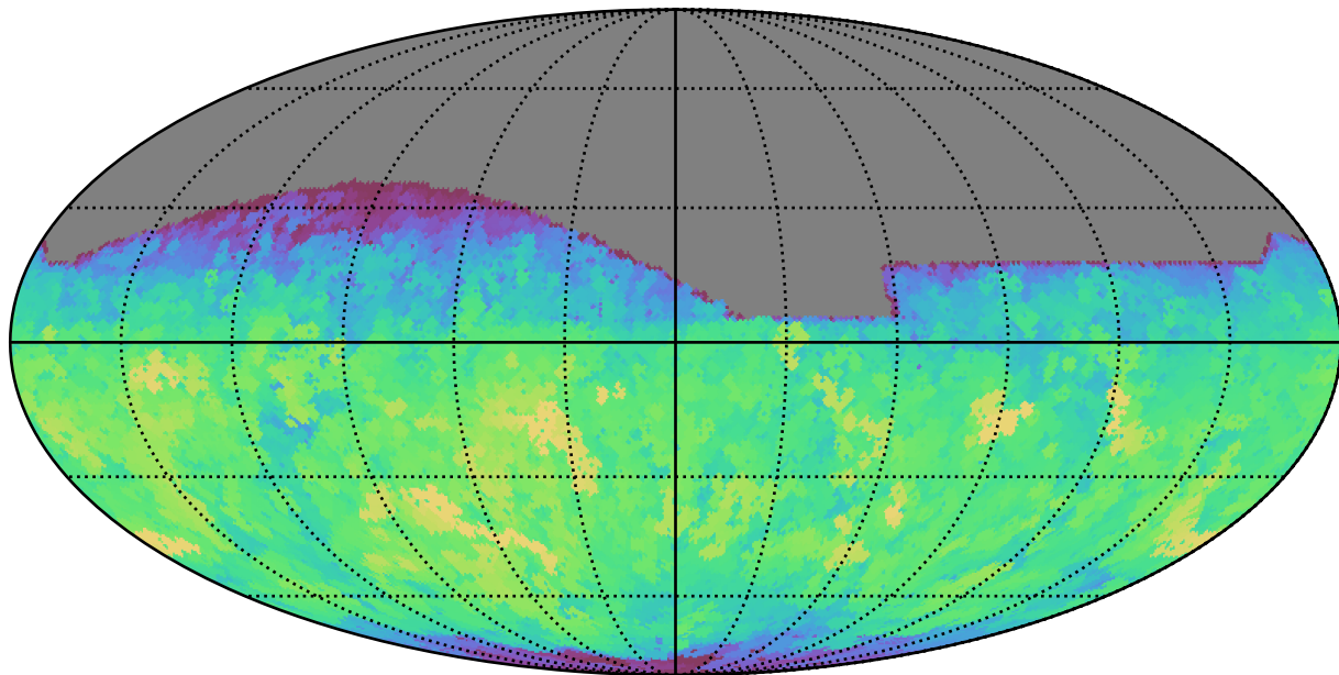
too_100_4v3.4_10yrs All sky i band: Max saturation_mag
