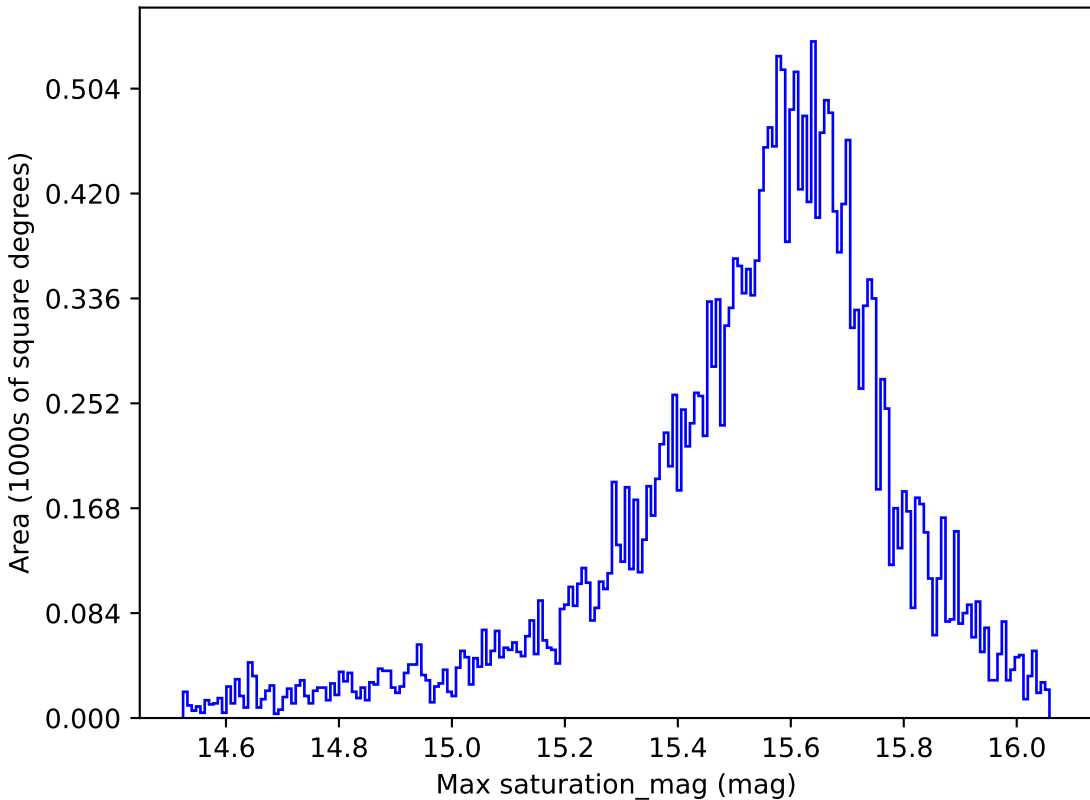
too_100_4v3.4_10yrs All sky i band: Max saturation_mag
