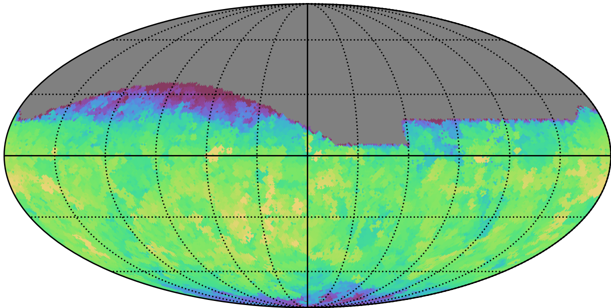
too_100_4v3.4_10yrs All sky g band: Max saturation_mag
