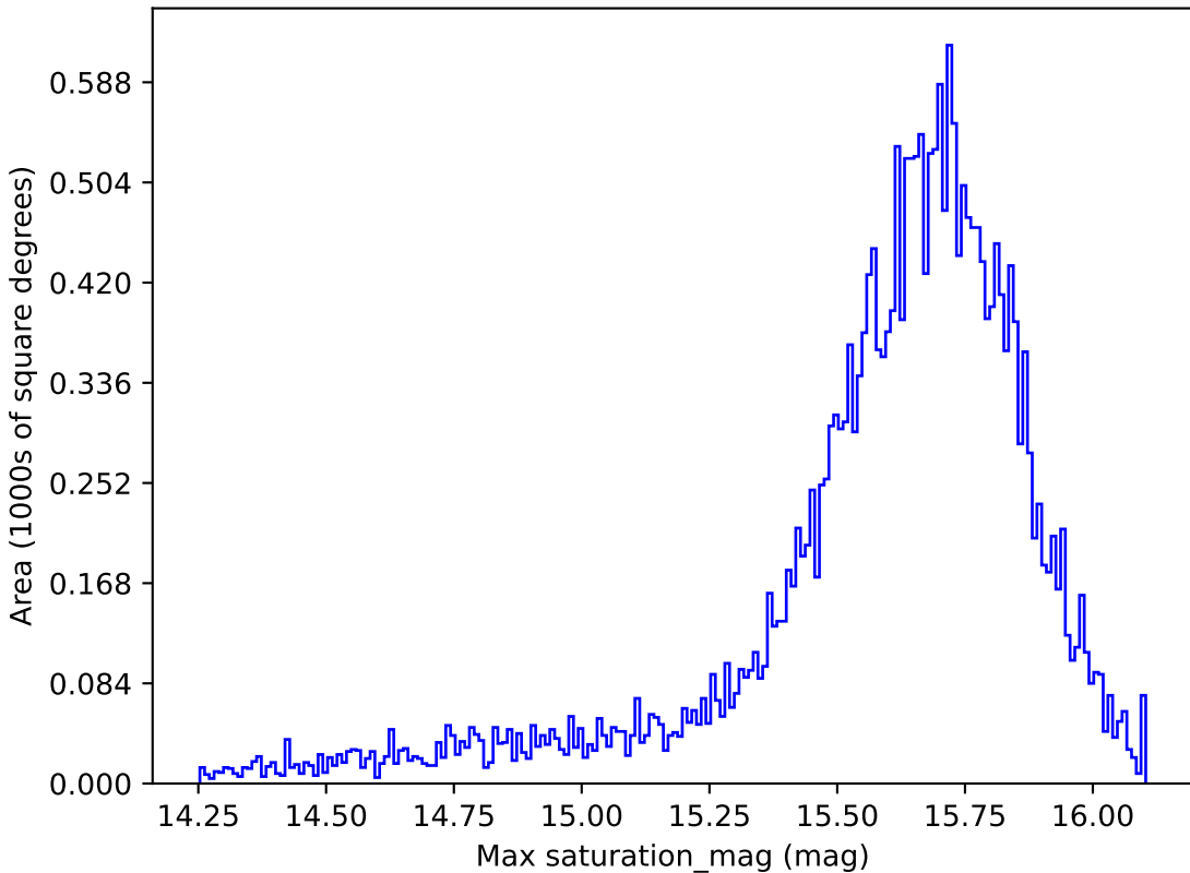
too_100_4v3.4_10yrs All sky g band: Max saturation_mag
