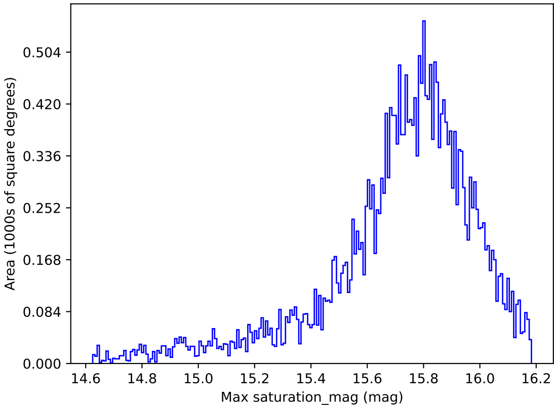
too_100_4v3.4_10yrs All sky all bands: Max saturation_mag
