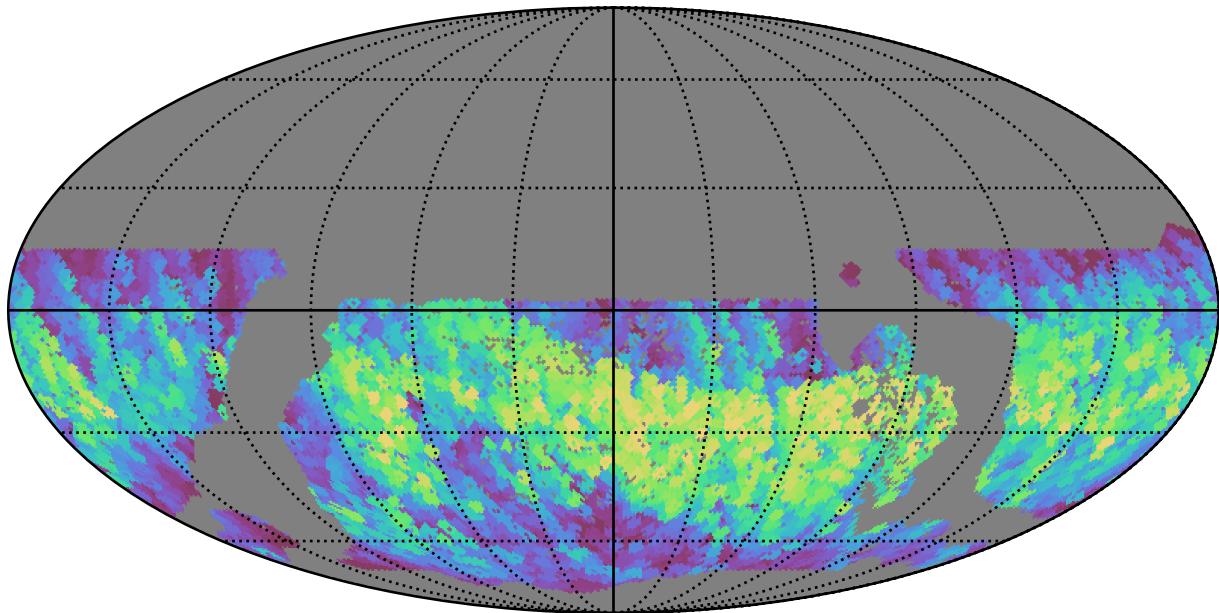
too_100_4v3.4_10yrs WFD z band: Max normairmass
