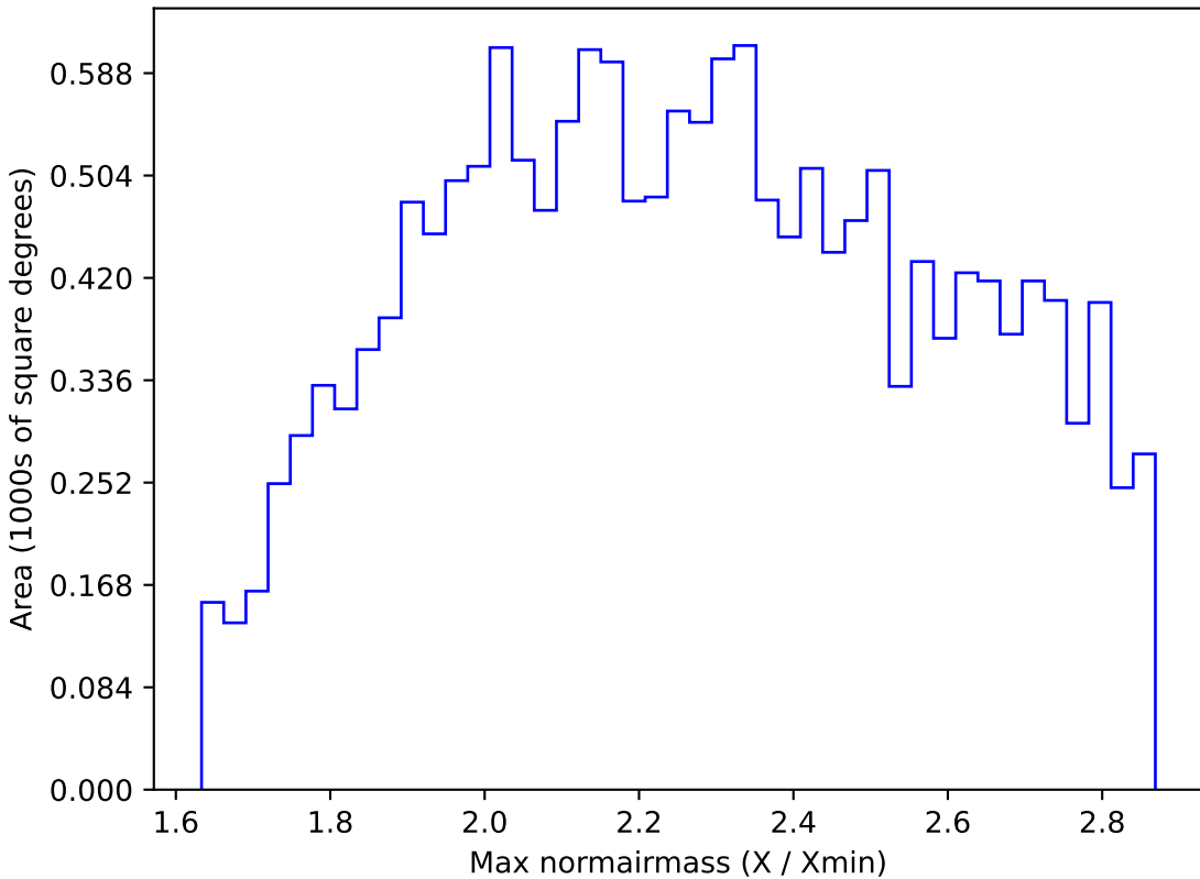
too_100_4v3.4_10yrs WFD z band: Max normairmass
