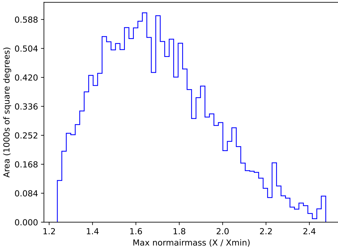
too_100_4v3.4_10yrs WFD u band: Max normairmass
