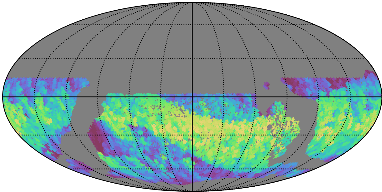
too_100_4v3.4_10yrs WFD i band: Max normairmass
