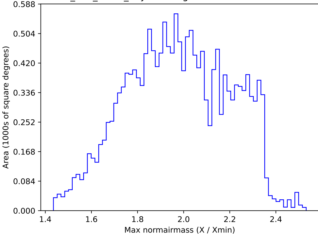
too_100_4v3.4_10yrs WFD g band: Max normairmass
