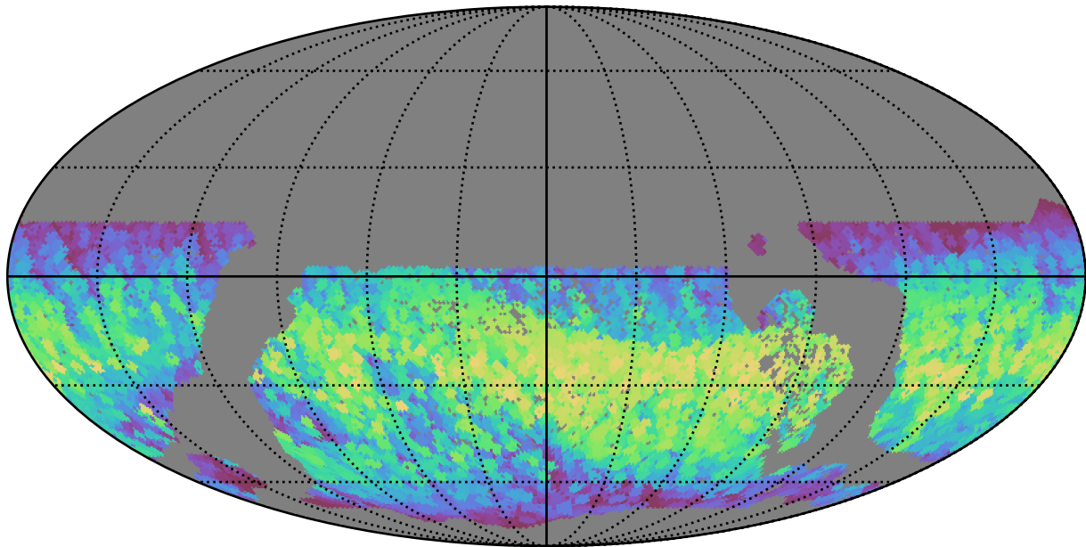
too_100_4v3.4_10yrs WFD all bands: Max normairmass
