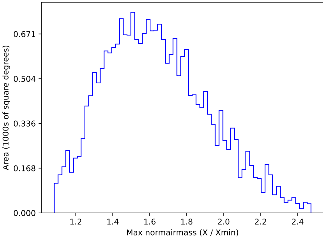
too_100_4v3.4_10yrs All sky u band: Max normairmass
