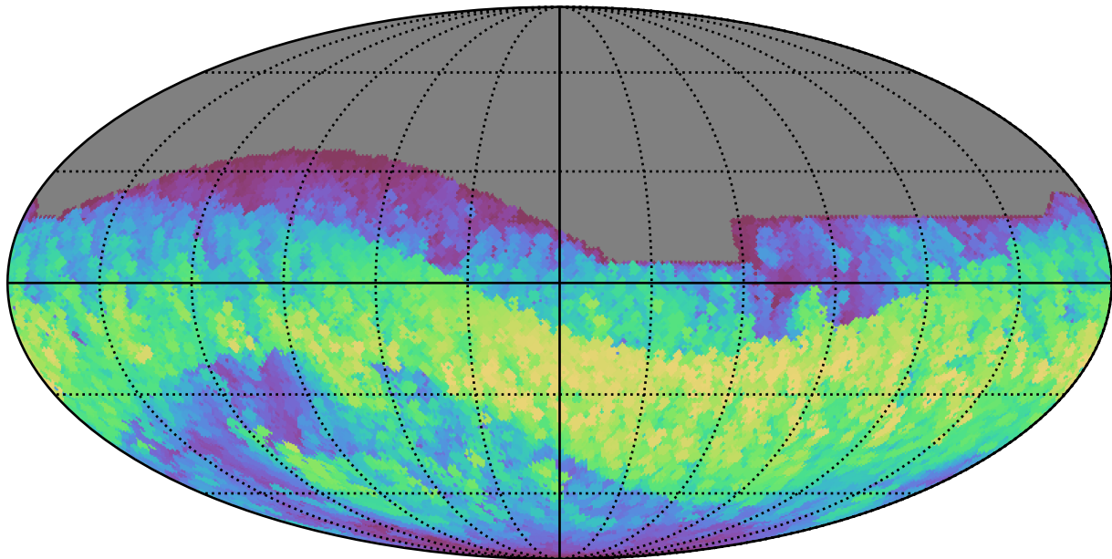
too_100_4v3.4_10yrs All sky i band: Max normairmass
