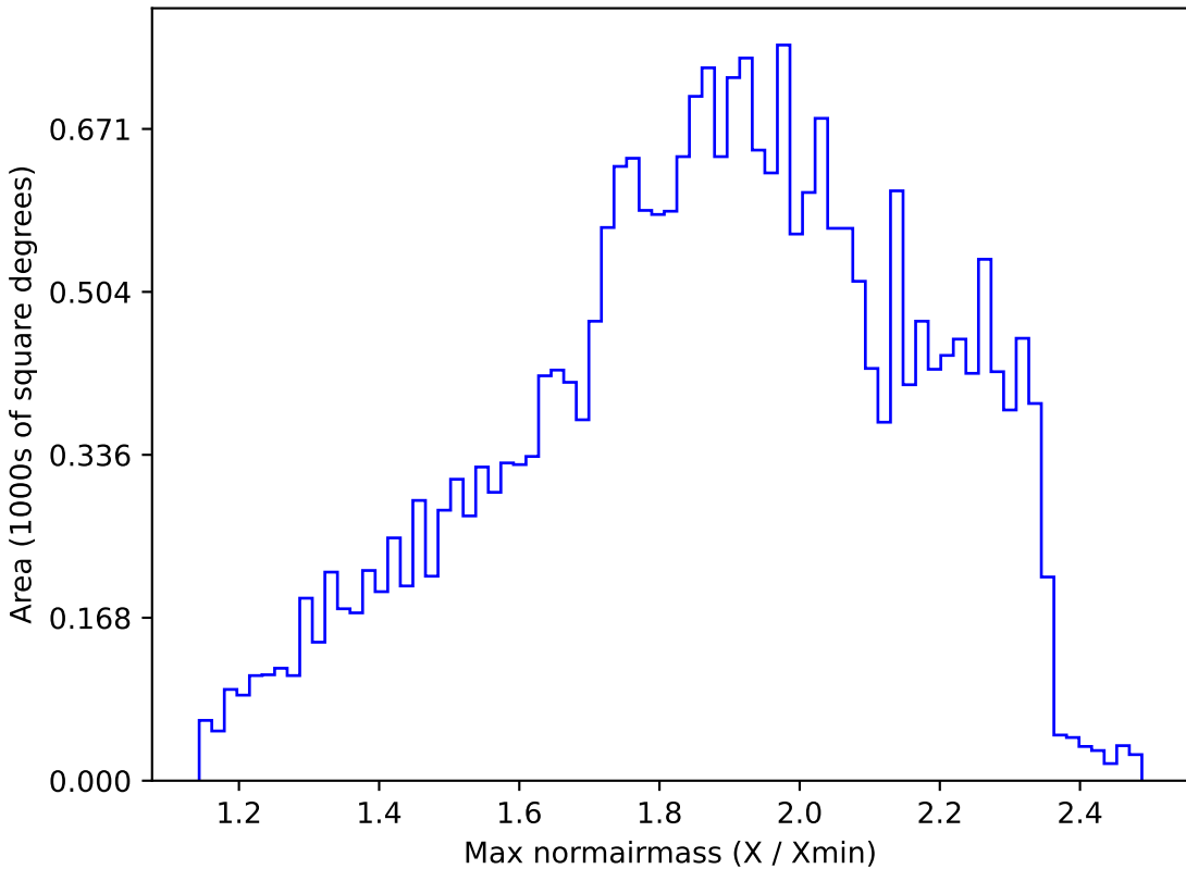
too_100_4v3.4_10yrs All sky g band: Max normairmass
