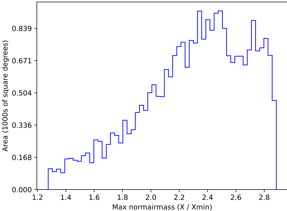
too_100_4v3.4_10yrs All sky all bands: Max normairmass
