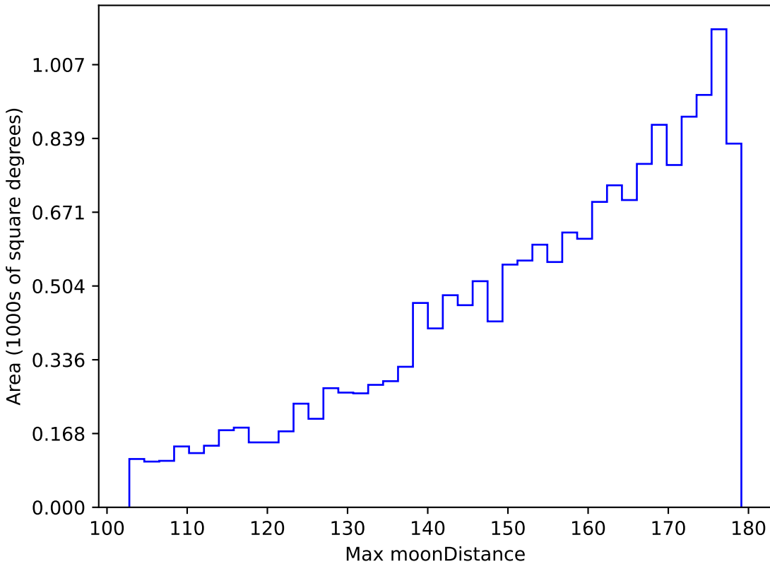
too_100_4v3.4_10yrs WFD z band: Max moonDistance
