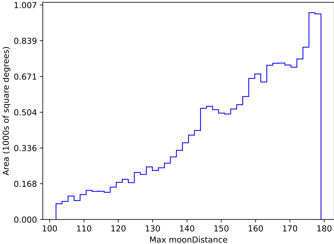
too_100_4v3.4_10yrs WFD u band: Max moonDistance
