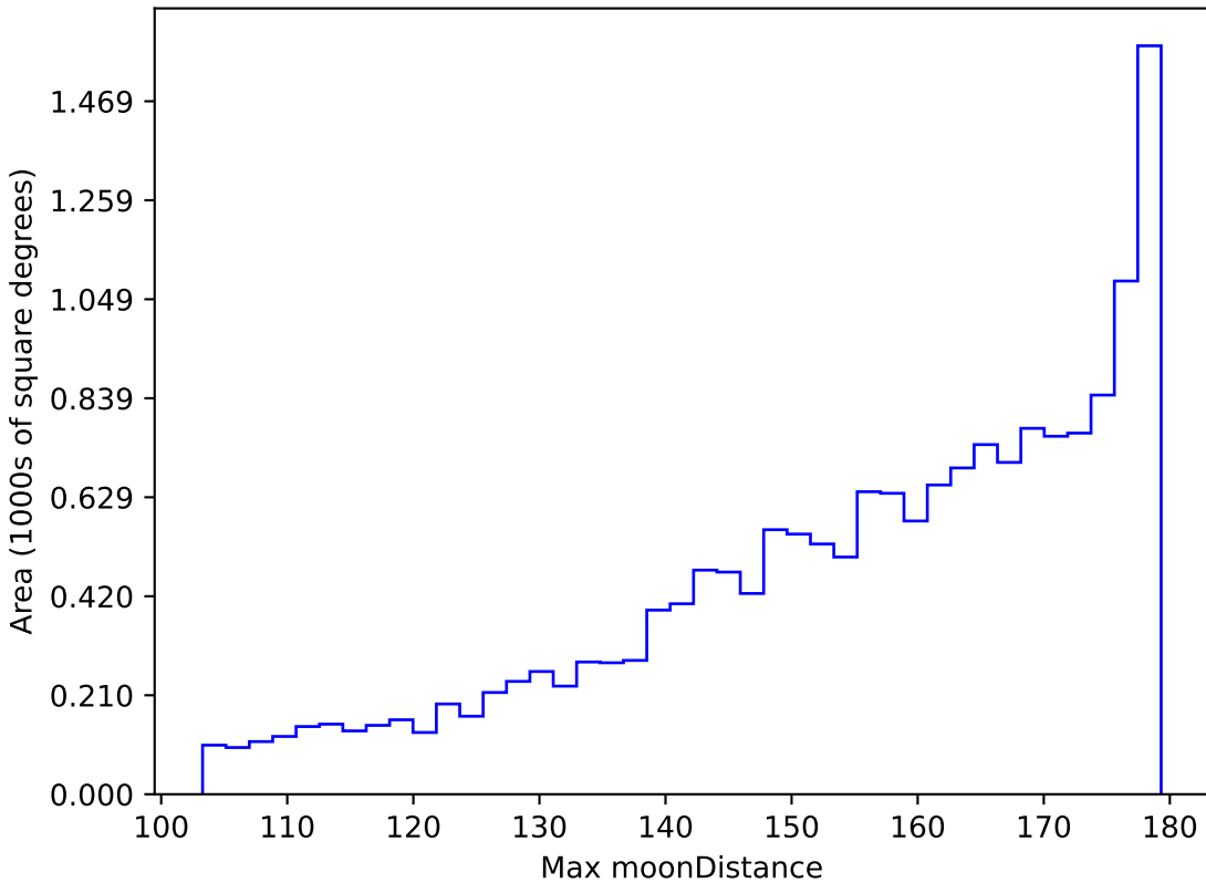
too_100_4v3.4_10yrs WFD r band: Max moonDistance
