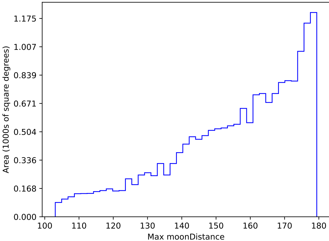
too_100_4v3.4_10yrs WFD i band: Max moonDistance
