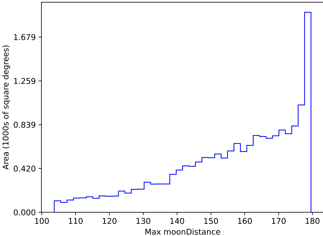
too_100_4v3.4_10yrs WFD all bands: Max moonDistance
