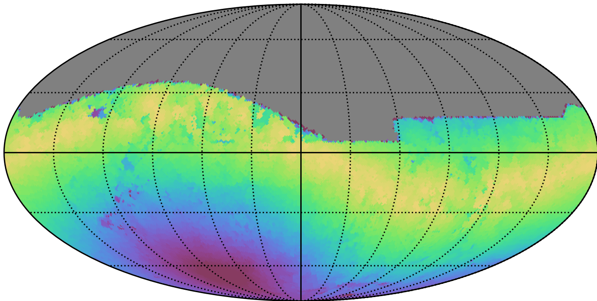
too_100_4v3.4_10yrs All sky z band: Max moonDistance
