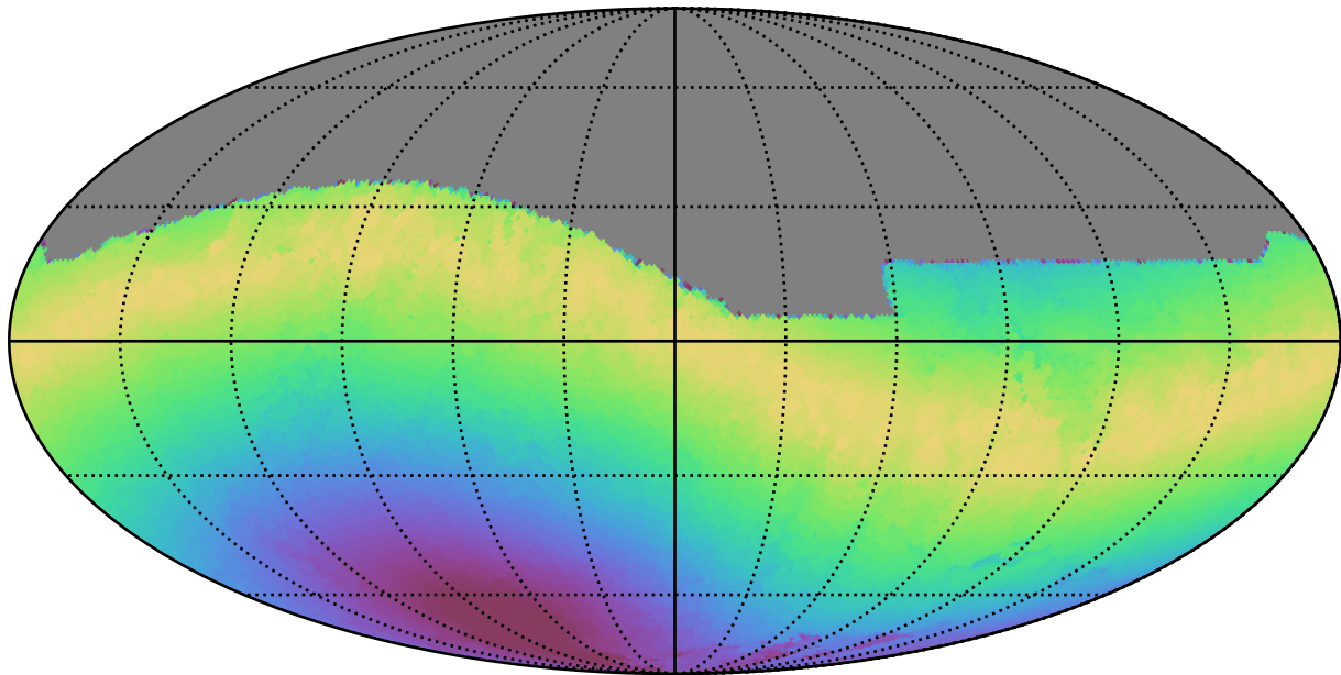
too_100_4v3.4_10yrs All sky r band: Max moonDistance
