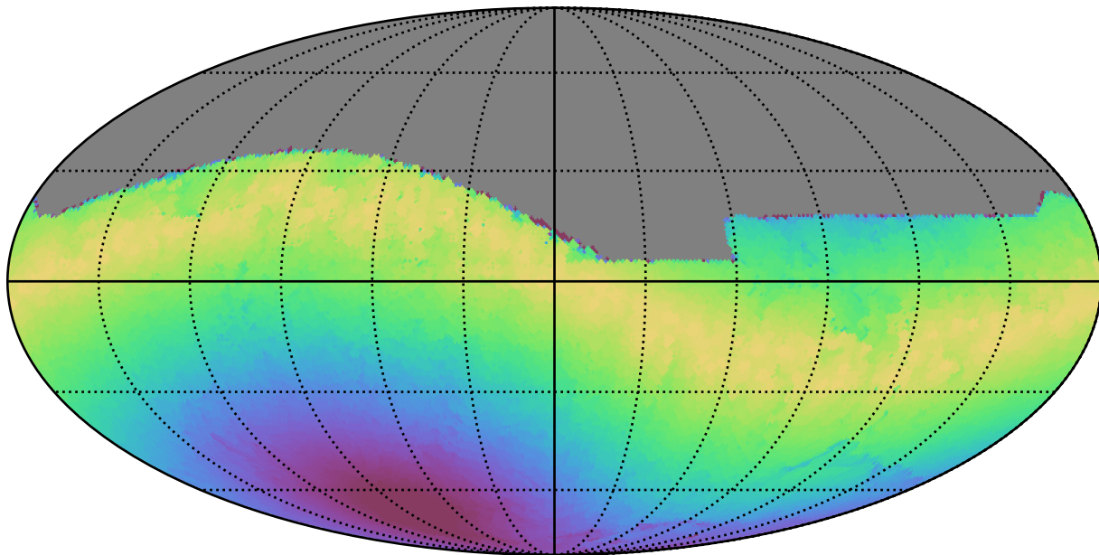
too_100_4v3.4_10yrs All sky i band: Max moonDistance
