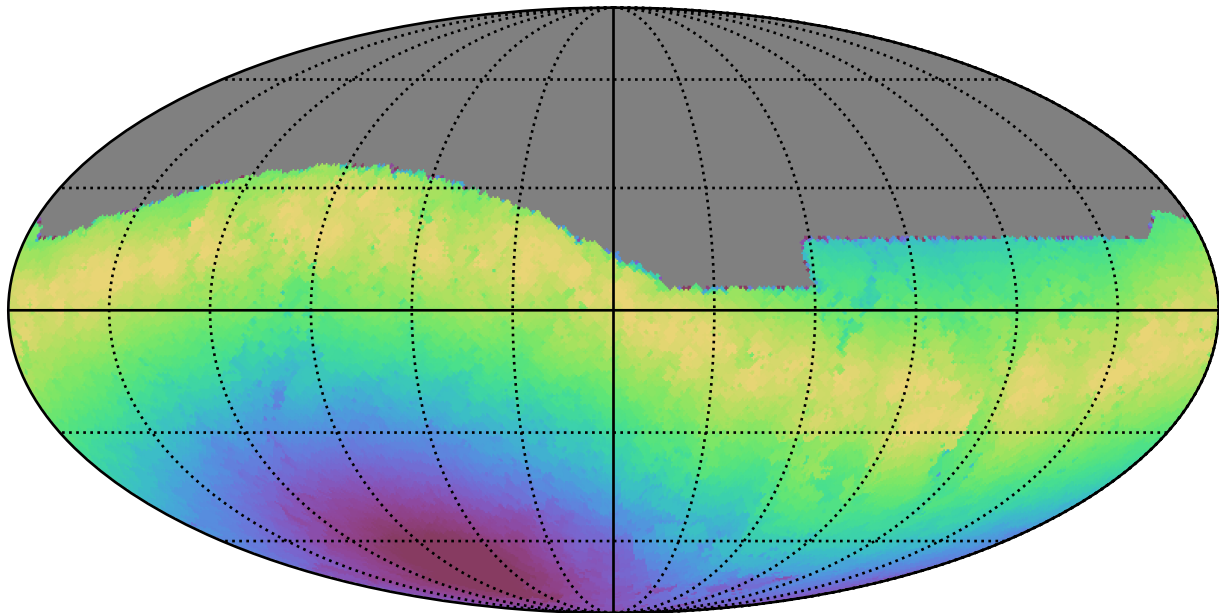
too_100_4v3.4_10yrs All sky g band: Max moonDistance
