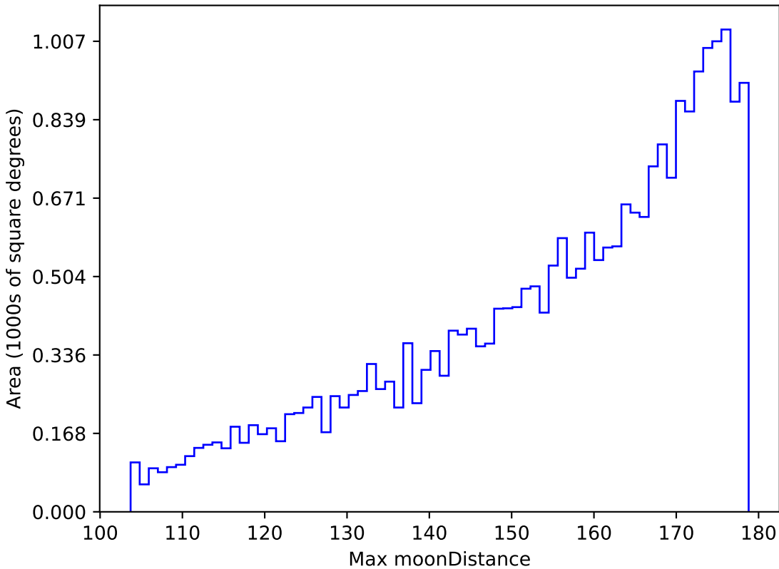
too_100_4v3.4_10yrs All sky g band: Max moonDistance
