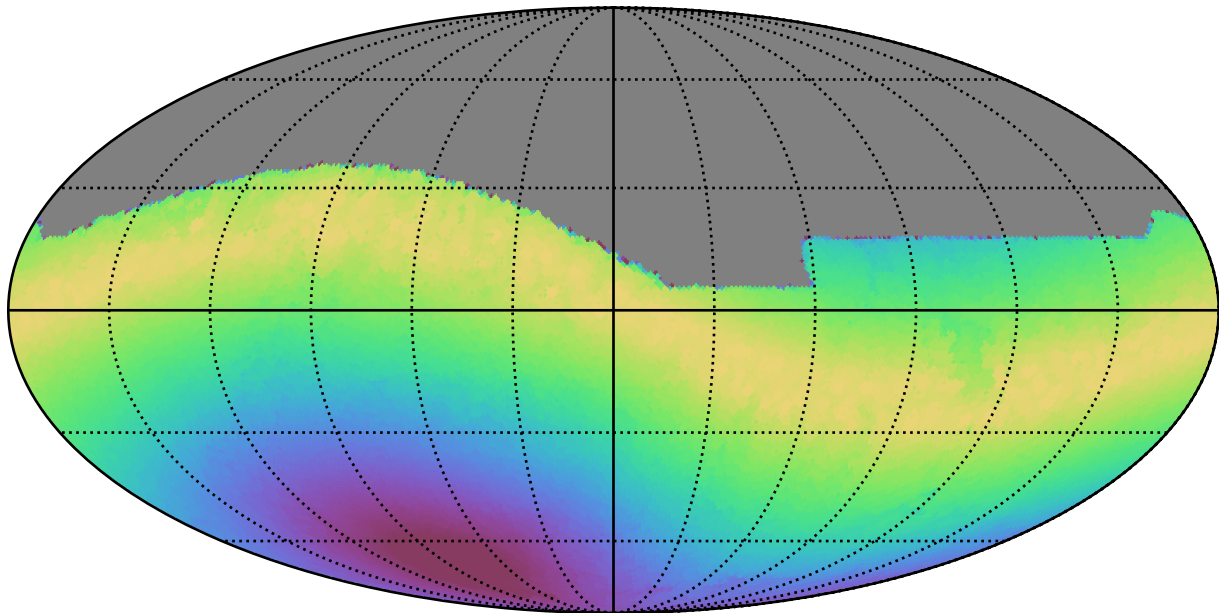
too_100_4v3.4_10yrs All sky all bands: Max moonDistance
