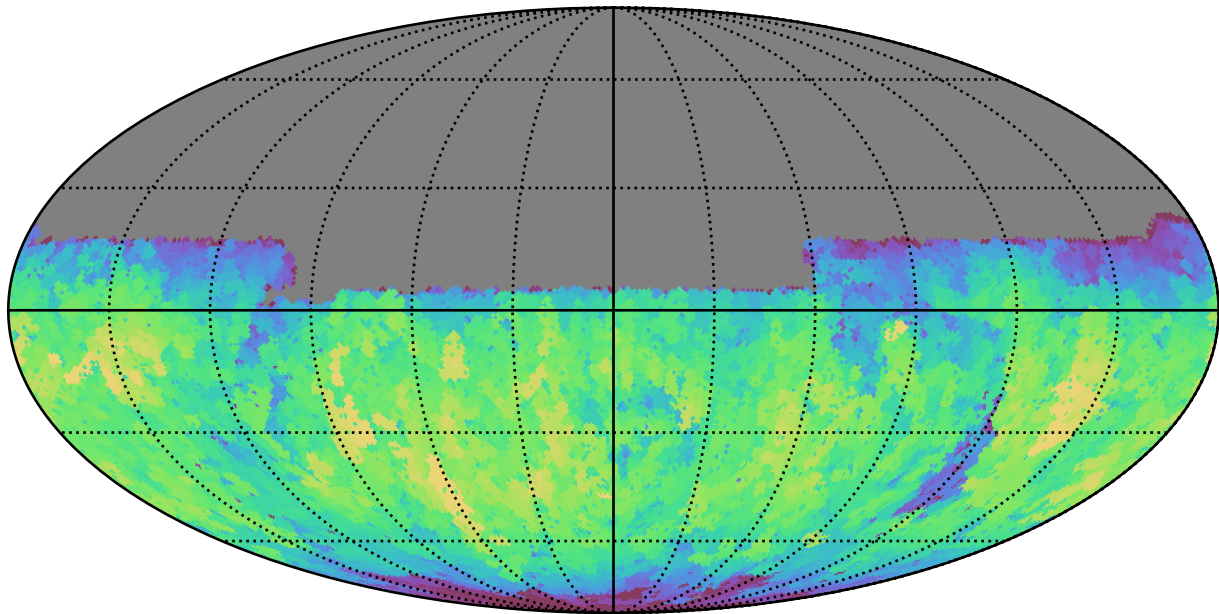
too_100_4v3.4_10yrs Yr 1 y band: Max fiveSigmaDepth
