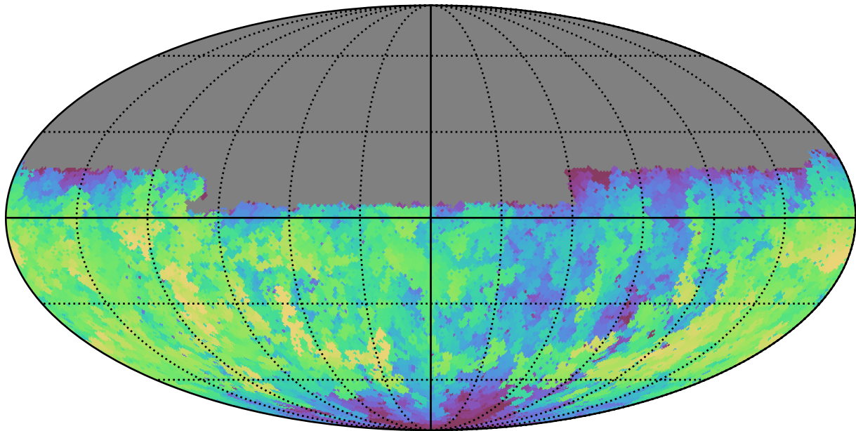
too_100_4v3.4_10yrs Yr 1 u band: Max fiveSigmaDepth
