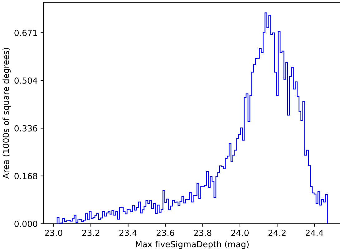
too_100_4v3.4_10yrs Yr 1 i band: Max fiveSigmaDepth
