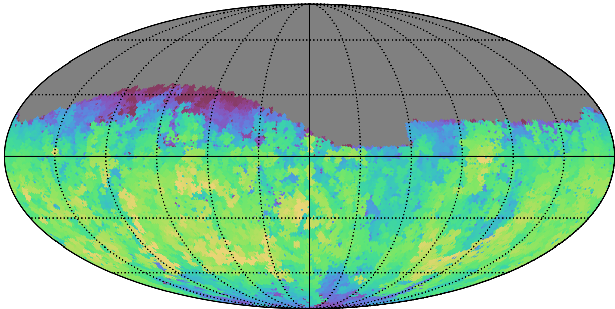
too_100_4v3.4_10yrs Yr 1 g band: Max fiveSigmaDepth
