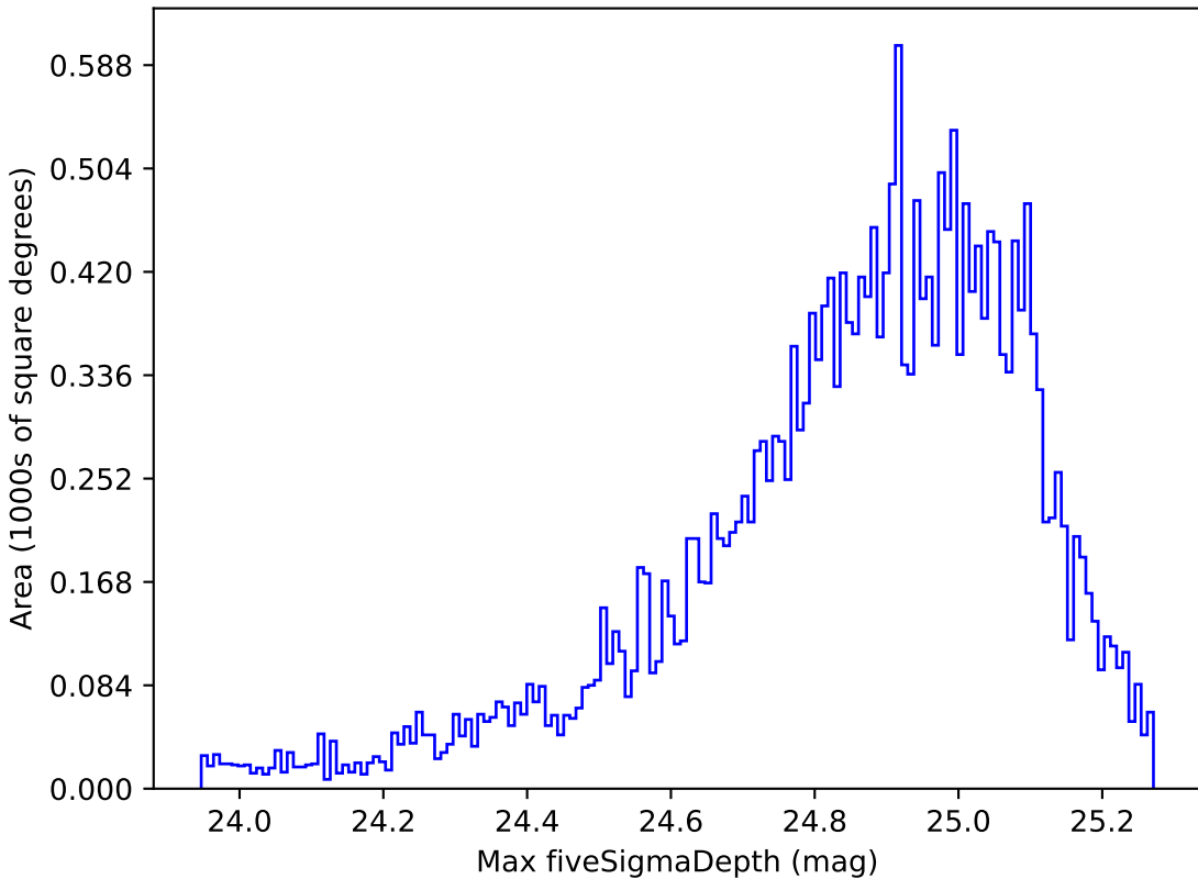
too_100_4v3.4_10yrs Yr 1 g band: Max fiveSigmaDepth
