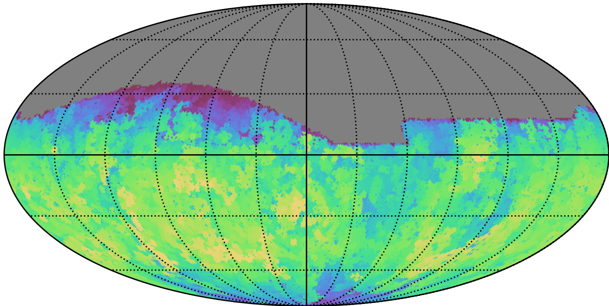
too_100_4v3.4_10yrs Yr 1 all bands: Max fiveSigmaDepth
