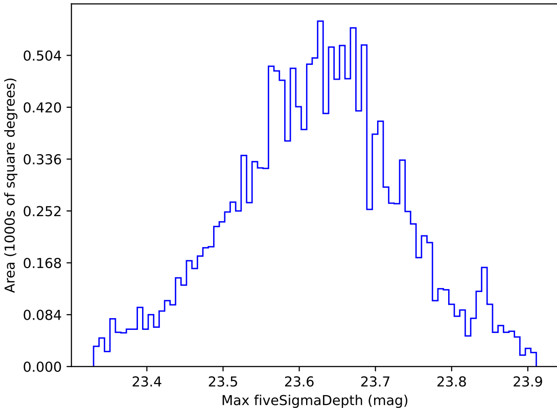
too_100_4v3.4_10yrs WFD z band: Max fiveSigmaDepth
