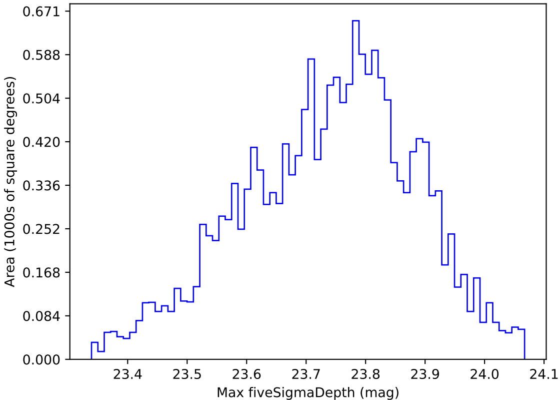
too_100_4v3.4_10yrs WFD u band: Max fiveSigmaDepth
