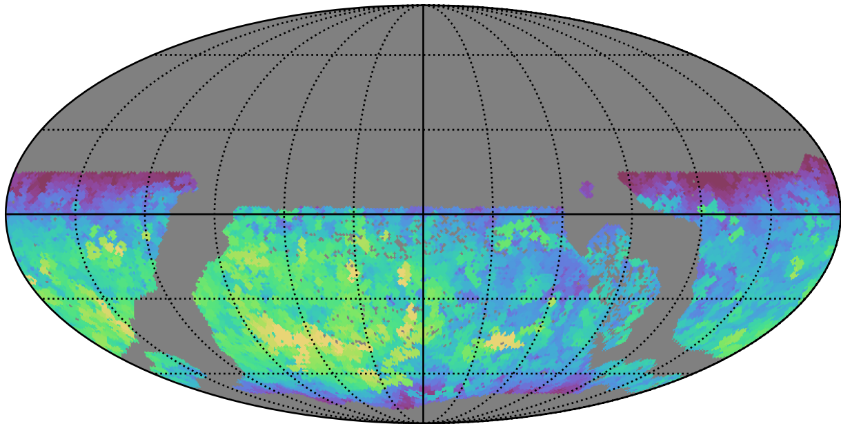
too_100_4v3.4_10yrs WFD r band: Max fiveSigmaDepth
