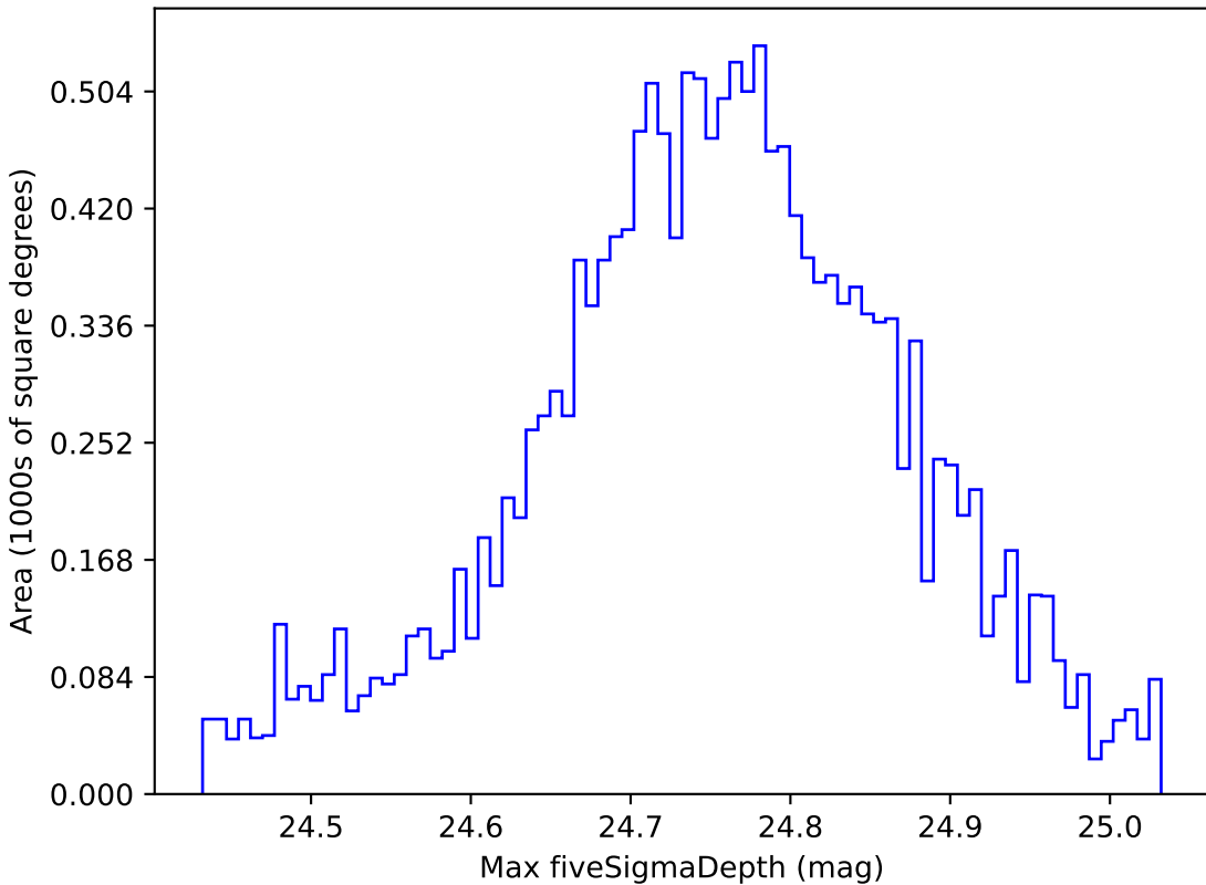
too_100_4v3.4_10yrs WFD r band: Max fiveSigmaDepth
