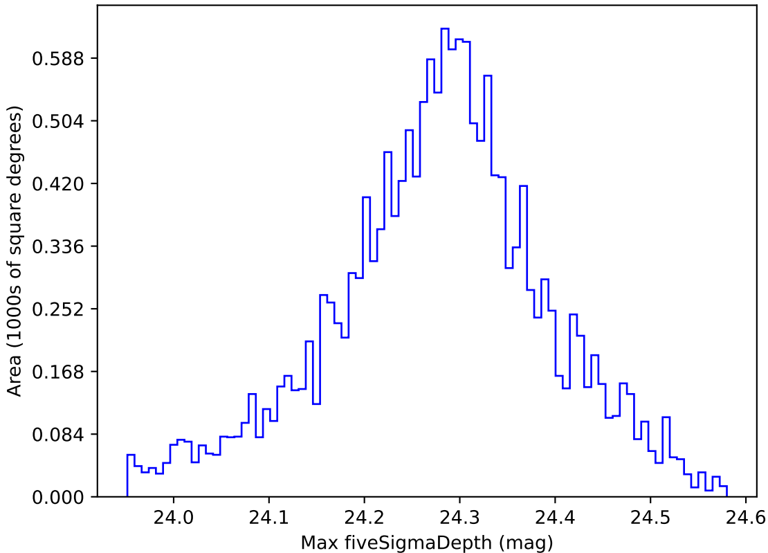
too_100_4v3.4_10yrs WFD i band: Max fiveSigmaDepth
