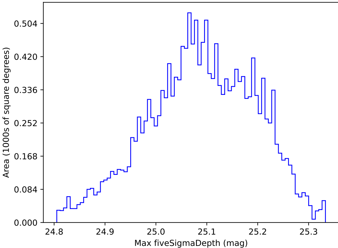
too_100_4v3.4_10yrs WFD g band: Max fiveSigmaDepth
