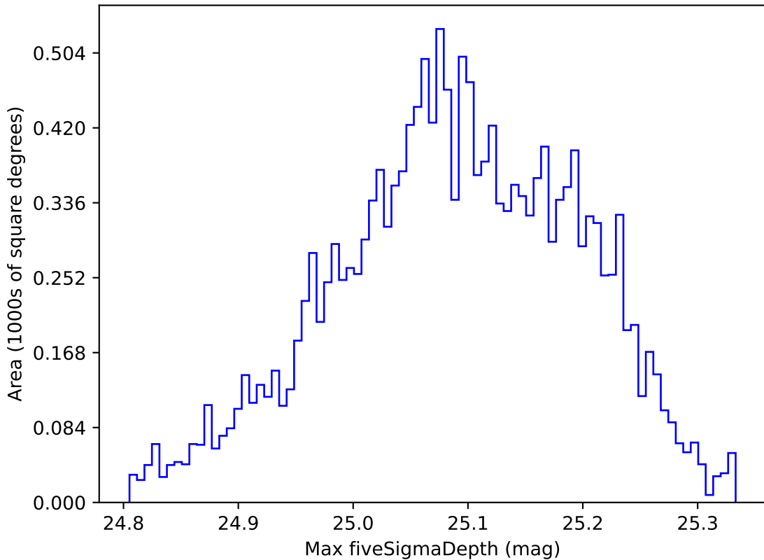
too_100_4v3.4_10yrs WFD all bands: Max fiveSigmaDepth
