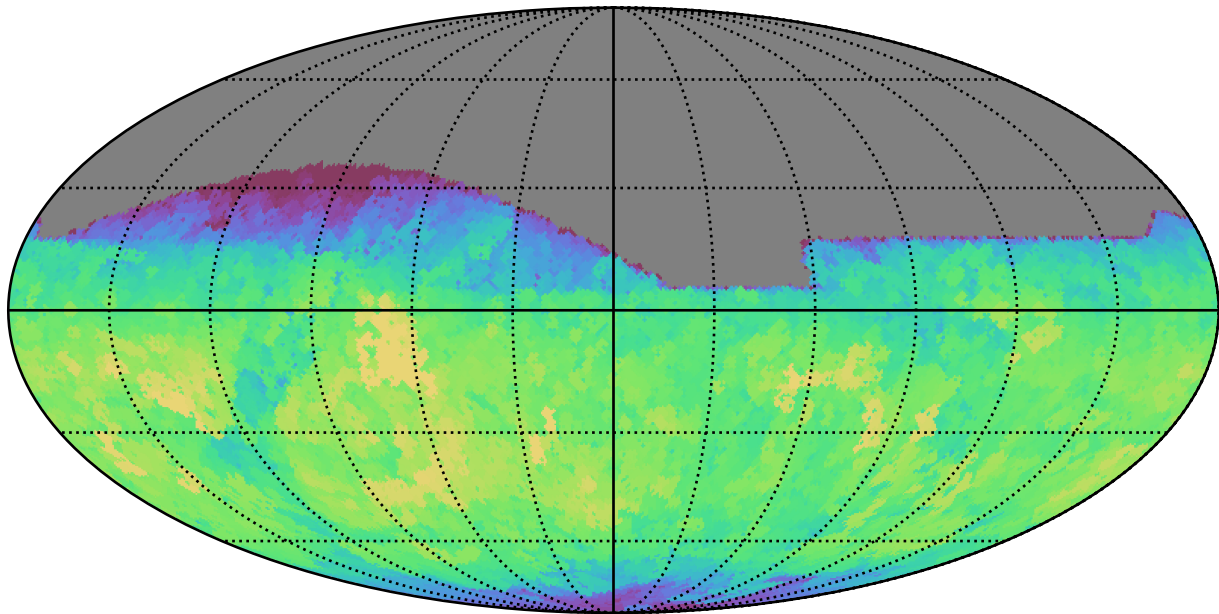
too_100_4v3.4_10yrs All sky z band: Max fiveSigmaDepth
