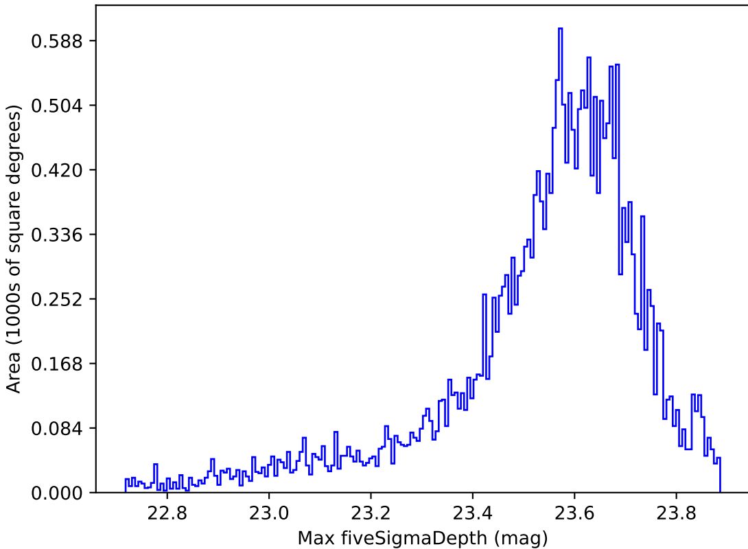
too_100_4v3.4_10yrs All sky z band: Max fiveSigmaDepth
