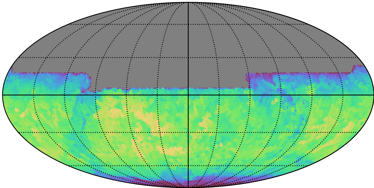
too_100_4v3.4_10yrs All sky y band: Max fiveSigmaDepth
