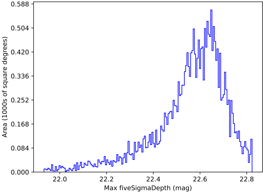
too_100_4v3.4_10yrs All sky y band: Max fiveSigmaDepth
