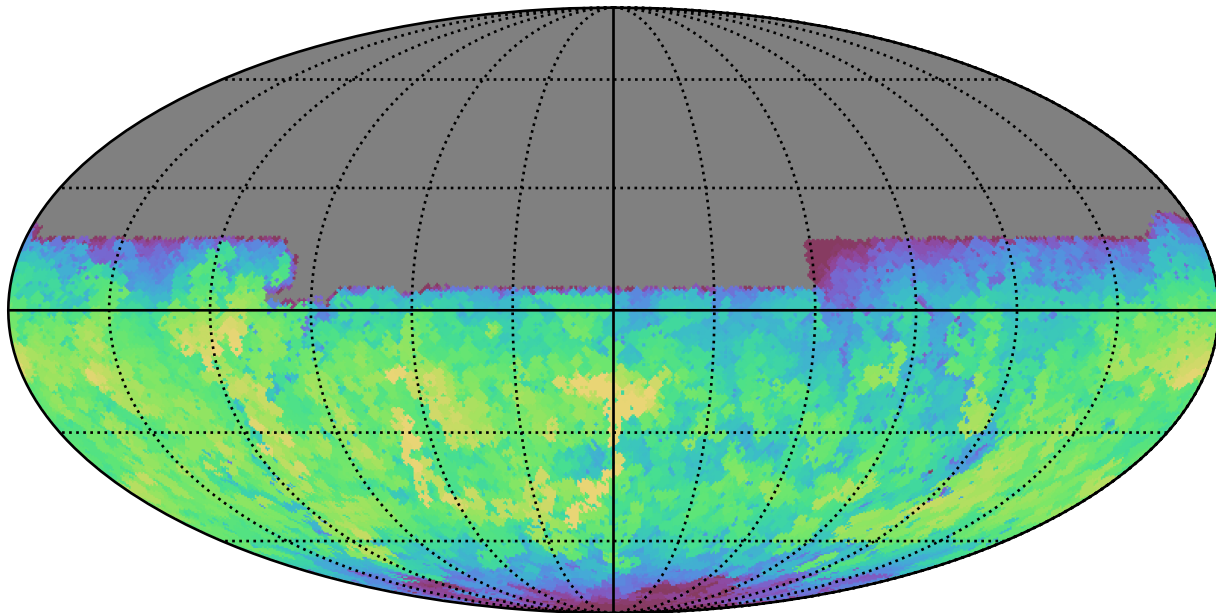
too_100_4v3.4_10yrs All sky u band: Max fiveSigmaDepth
