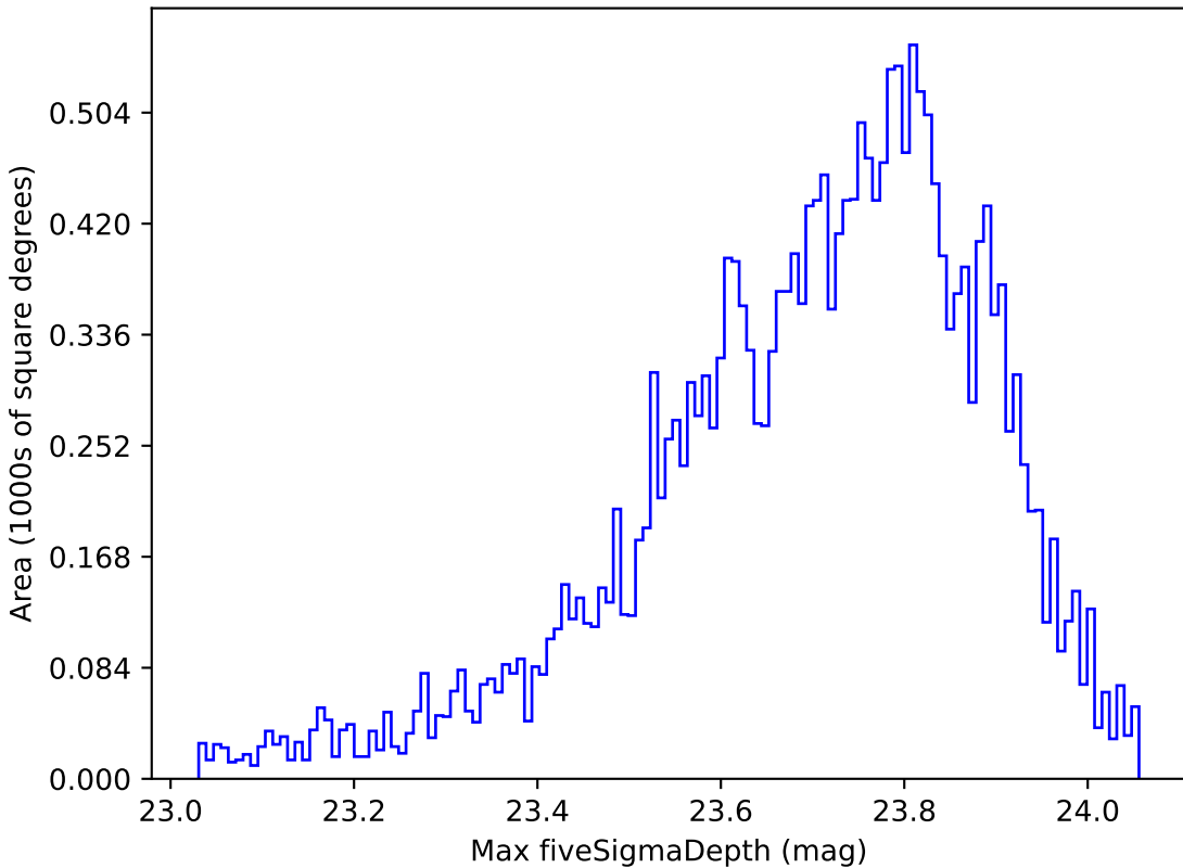
too_100_4v3.4_10yrs All sky u band: Max fiveSigmaDepth
