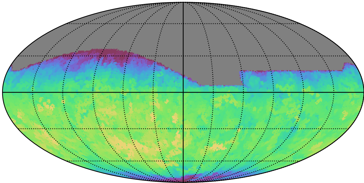
too_100_4v3.4_10yrs All sky r band: Max fiveSigmaDepth
