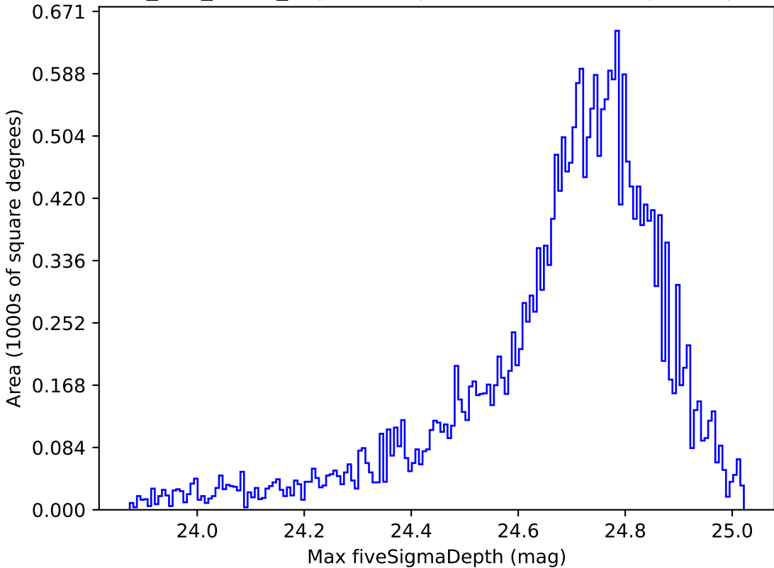
too_100_4v3.4_10yrs All sky r band: Max fiveSigmaDepth
