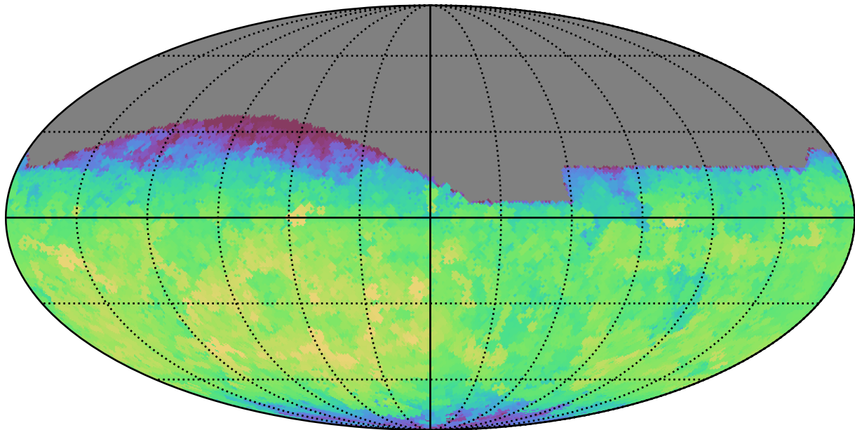
too_100_4v3.4_10yrs All sky g band: Max fiveSigmaDepth
